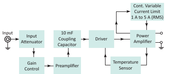
Fig. 1 Simplified block diagram of Power Amplifier Type 2718
