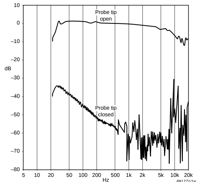
Fig.3 Comparison of typical sensitivities with probe tip opened (upper curve) and closed in 1 \text{ m}^3 rigid cavity (lower curve)
