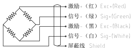
接线图Wiring Schematic Diagram
